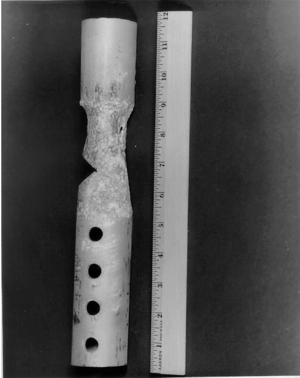
Figure 5-2 Galvanic corrosion on aluminum leg of 129ft tower.
